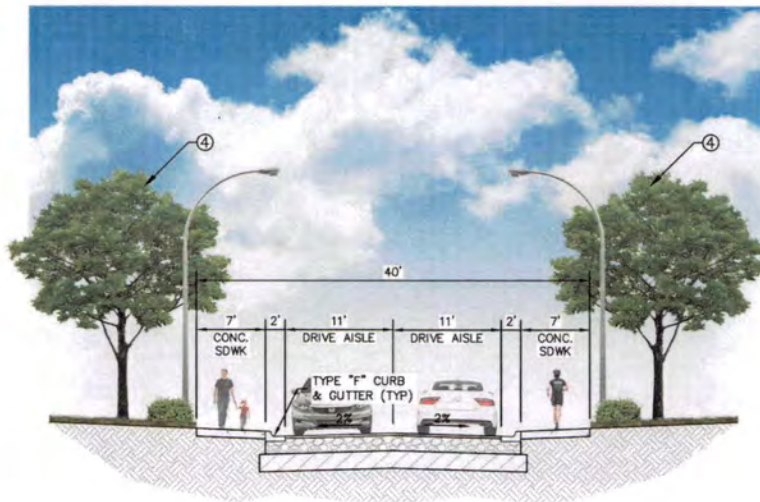
SECTION D-D (ENTRY DRIVE) N.T.S
