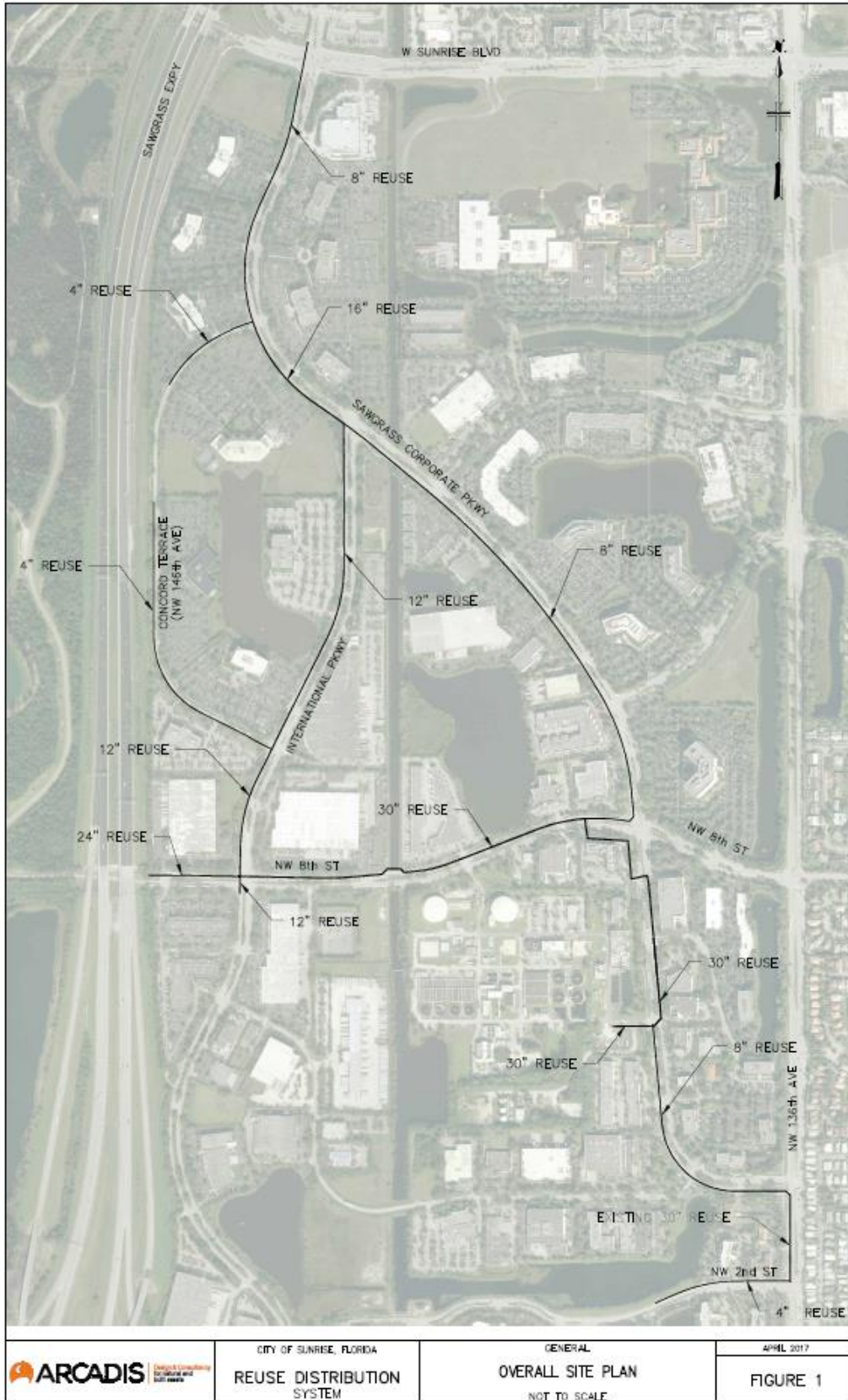
Figure 1. City of Sunrise Proposed Reuse Distribution System
