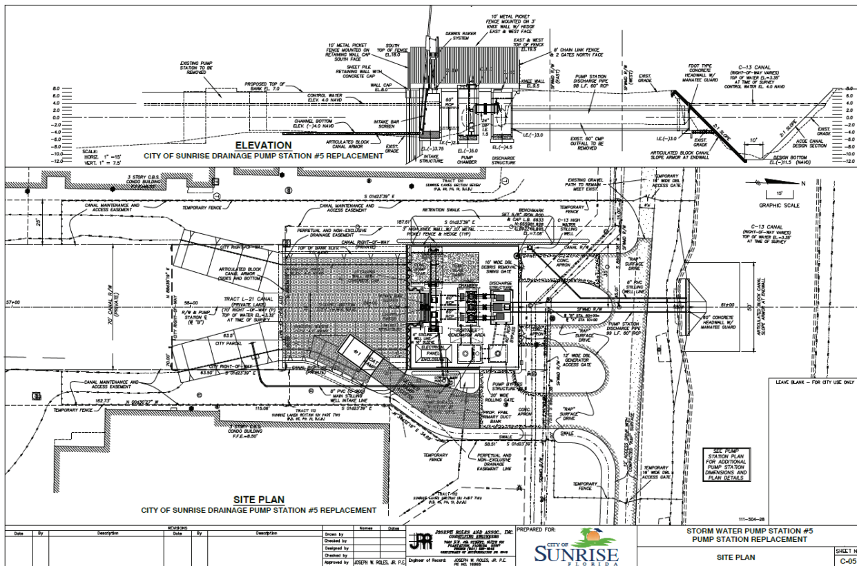
Figure 2. Site Plan
